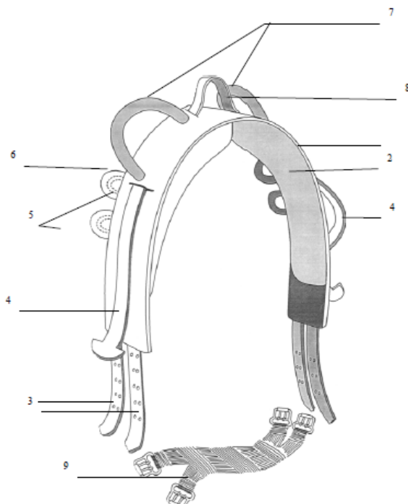
1. Outside surface 2. Leather padding 3. Girth straps 4. Foot straps 5. Rings for side reins 6. Leather covering of rings 7. Grips (shape of the grips are not defined) 8. Auxiliary holding strap 9. Girth
